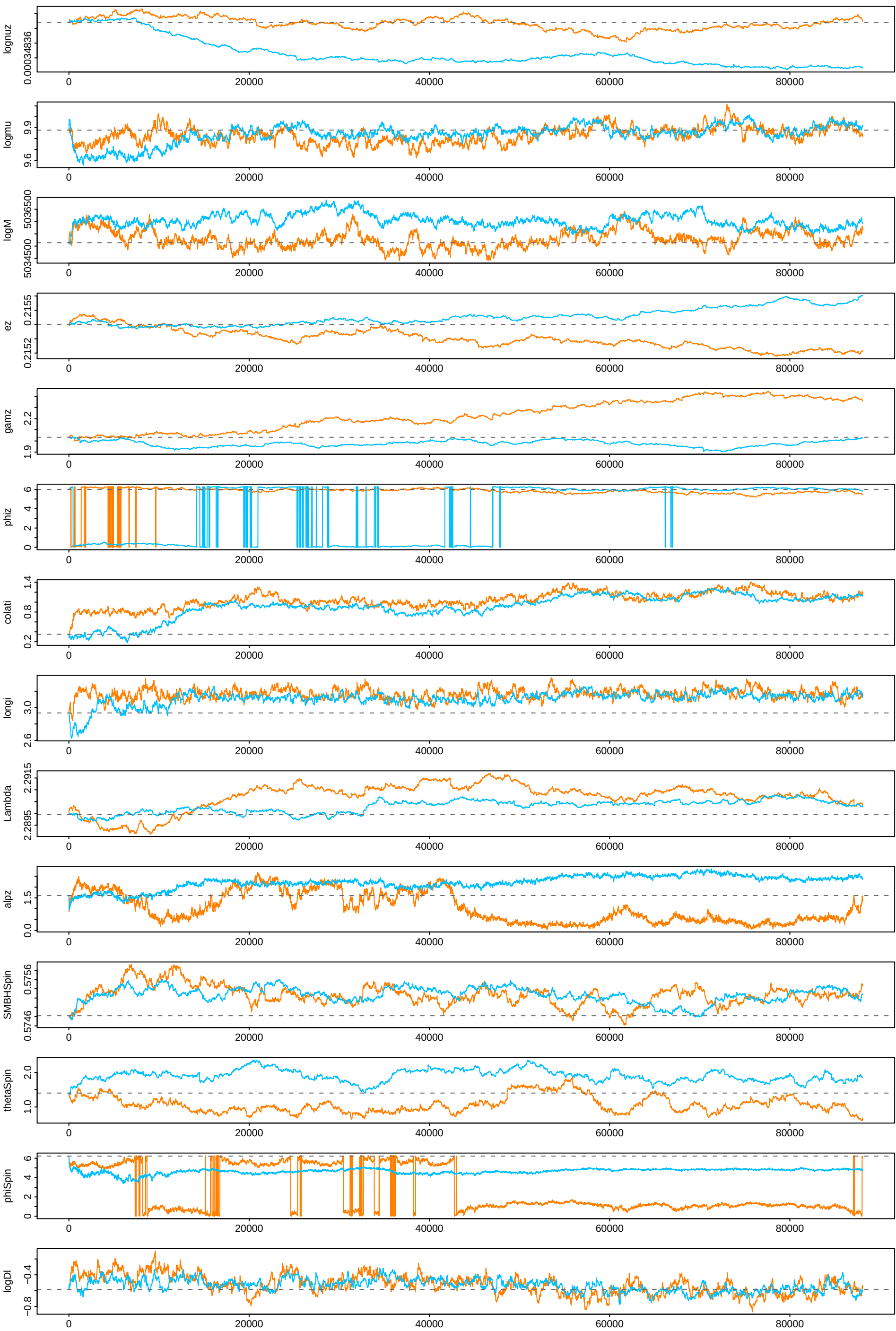
45 Days data segment (2^18 data points): non-mpi: cold vs heated chain
