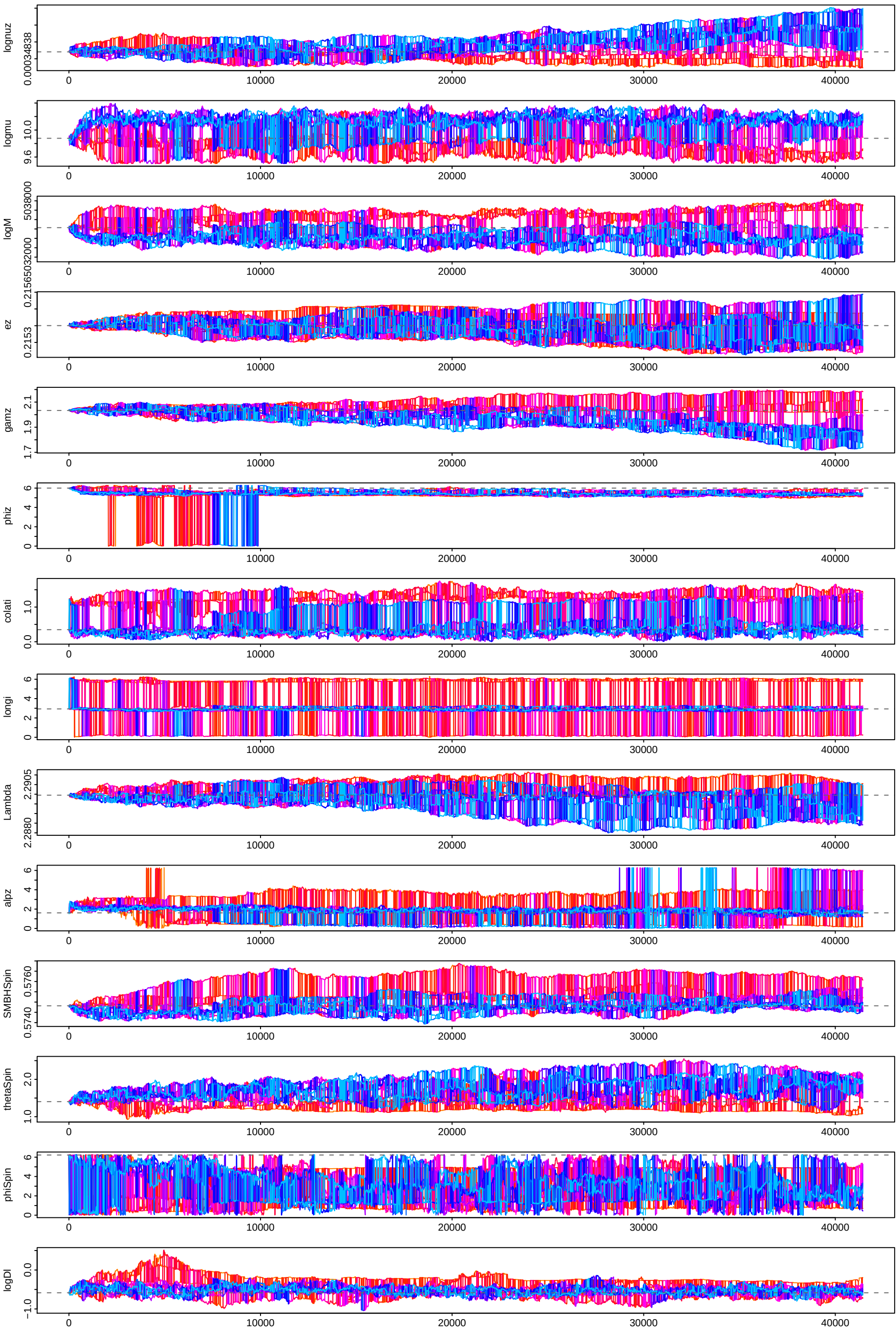
45 Days data segment (2^18 data points): 10 chains mpi: all 10 chains
