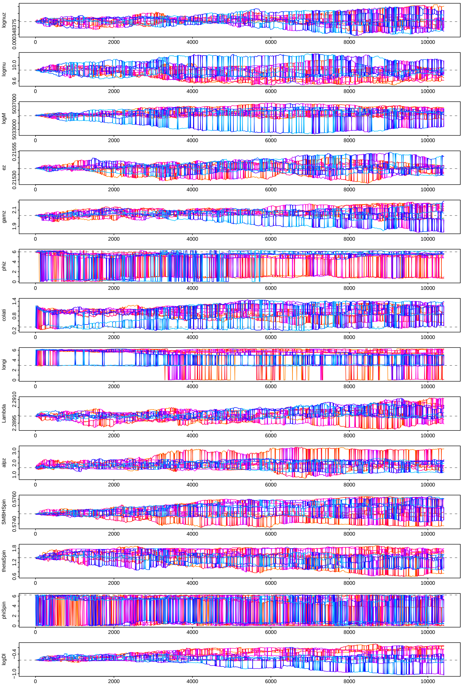
45 Days data segment (2^18 data points): 10 chains mpi: all 10 chains: Updated Proposal Covariance Matrix
