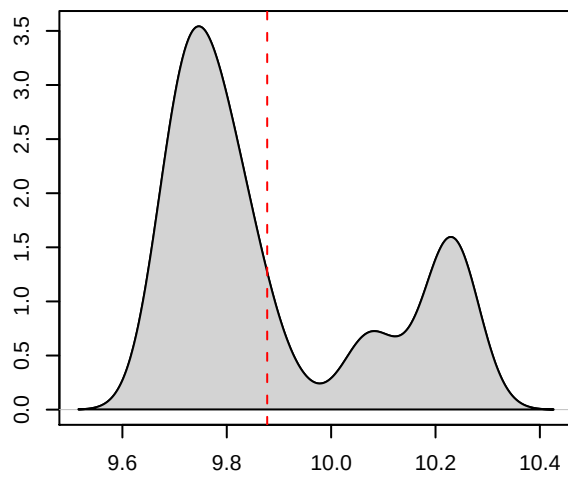
Density Plots
