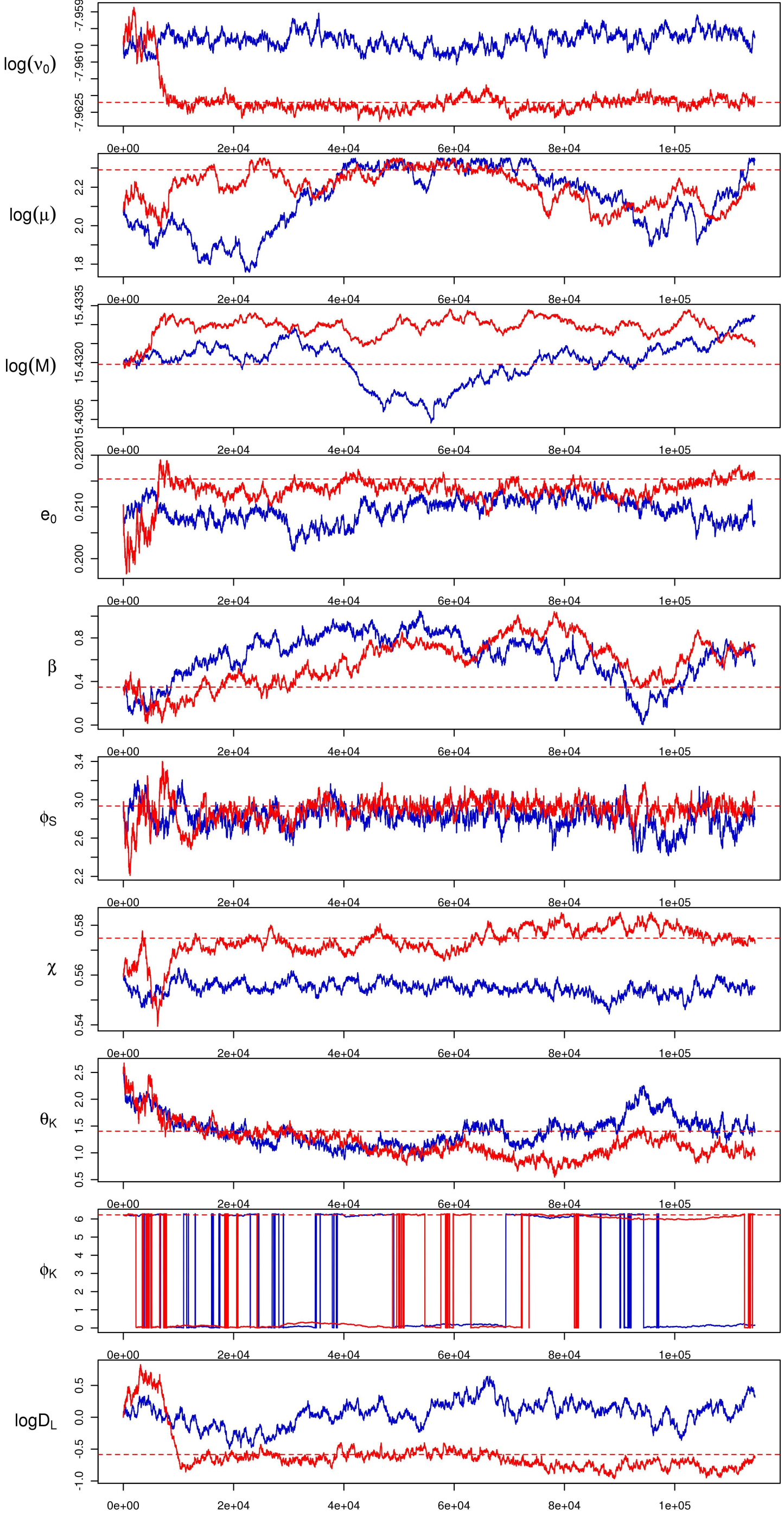
First Signal: 2 Chain Parrallel MCMC: Trace plots for both chains (Red=Hot, Blue=Cold)
