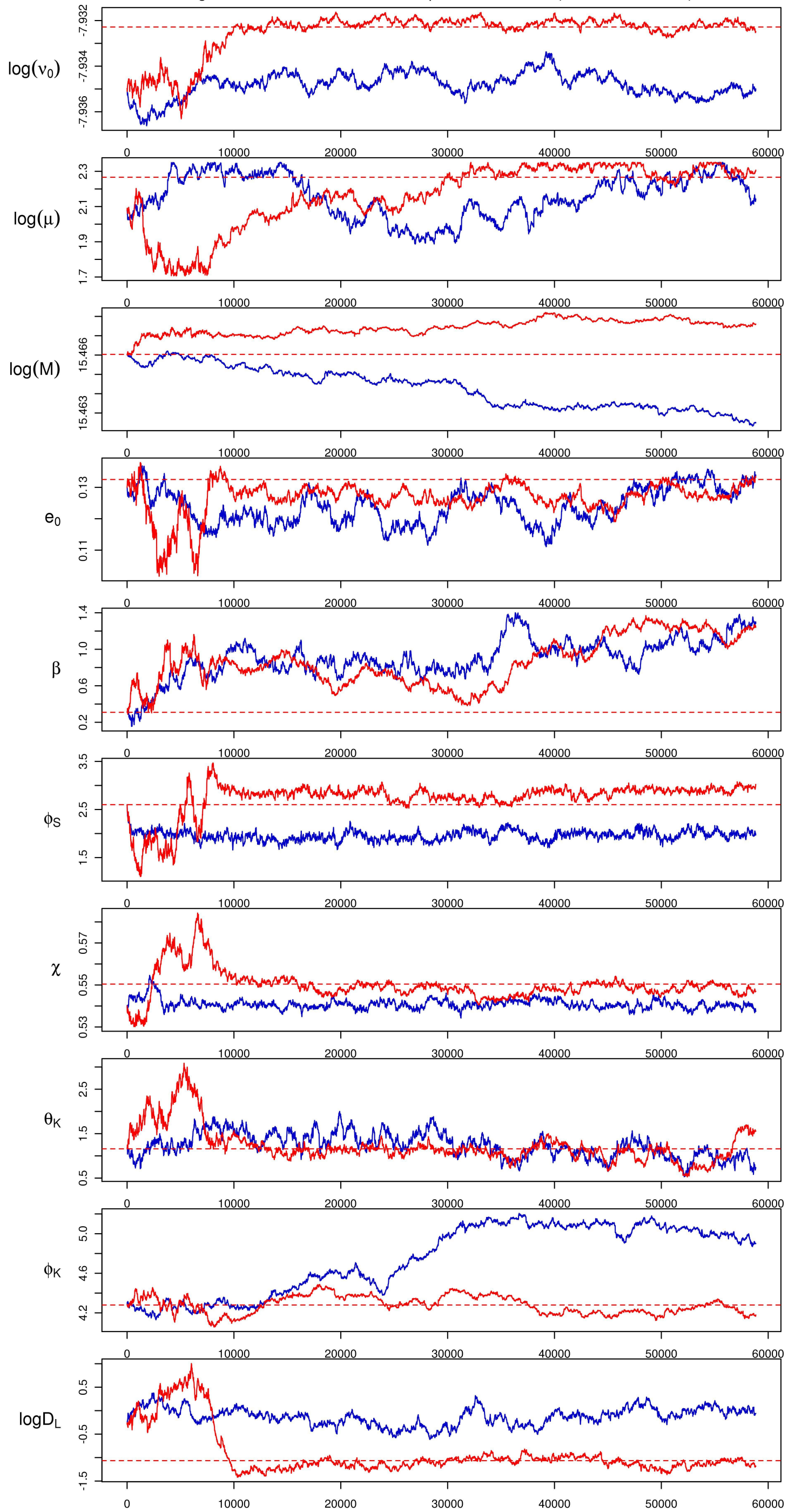
Second Signal: 2 Chain Parrallel MCMC: Trace plots for both chains (Red=Hot, Blue=Cold)
