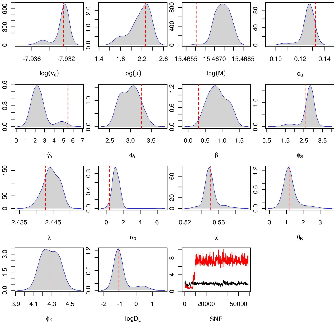
Second Signal: 2 Chain Parallel MCMC: Density plots for the hot chain
