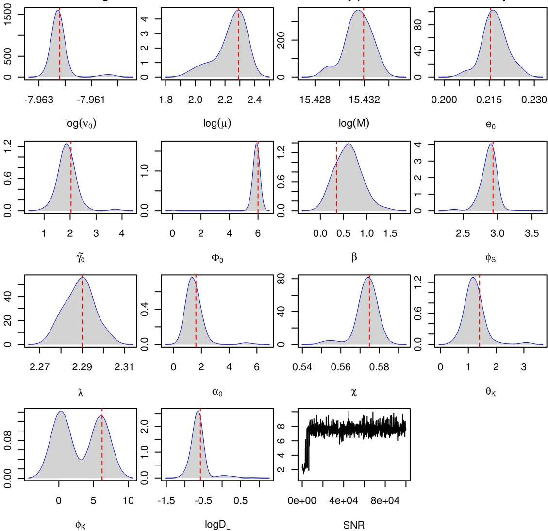
First Signal: 30 Chains Parallel MPI MCMC: Density plots for the cold chain only
