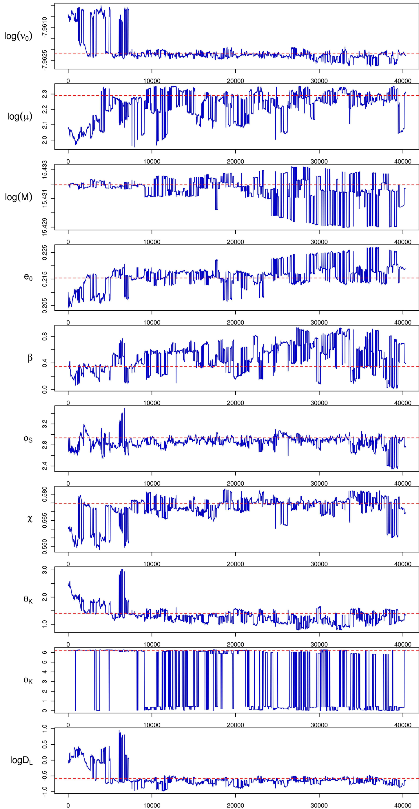
First Signal: 30 Chains Parallel MPI MCMC: Trace plots for cold chain only
