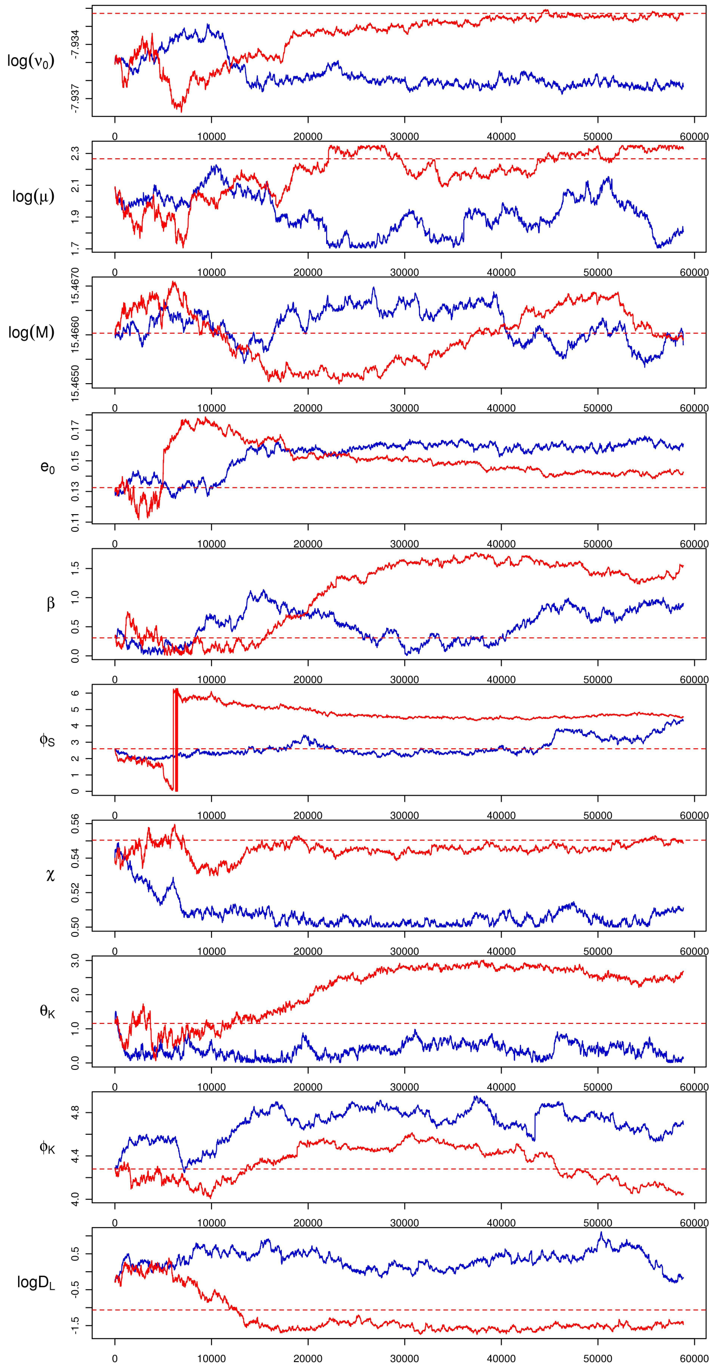
Second Signal: 2 Chain Parallel MCMC: Trace plots for both chains (Red=Hot, Blue=Cold)
