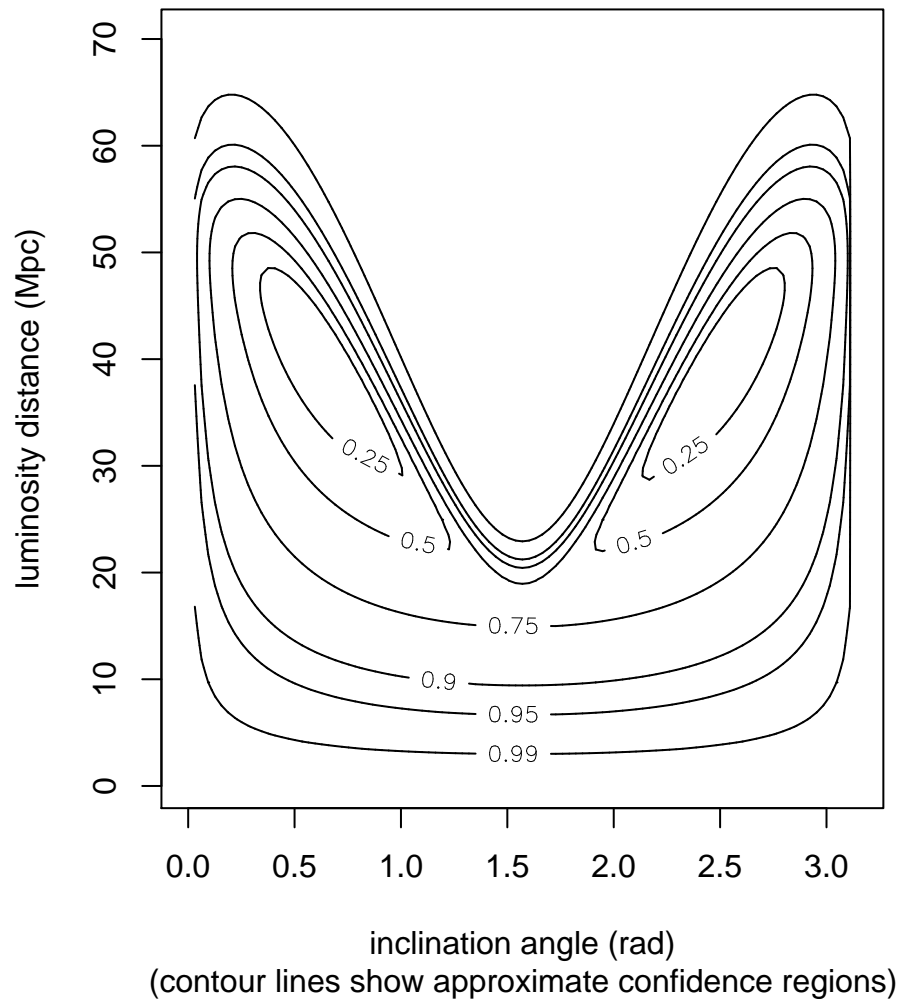
marginal prior density (for fixed masses)
