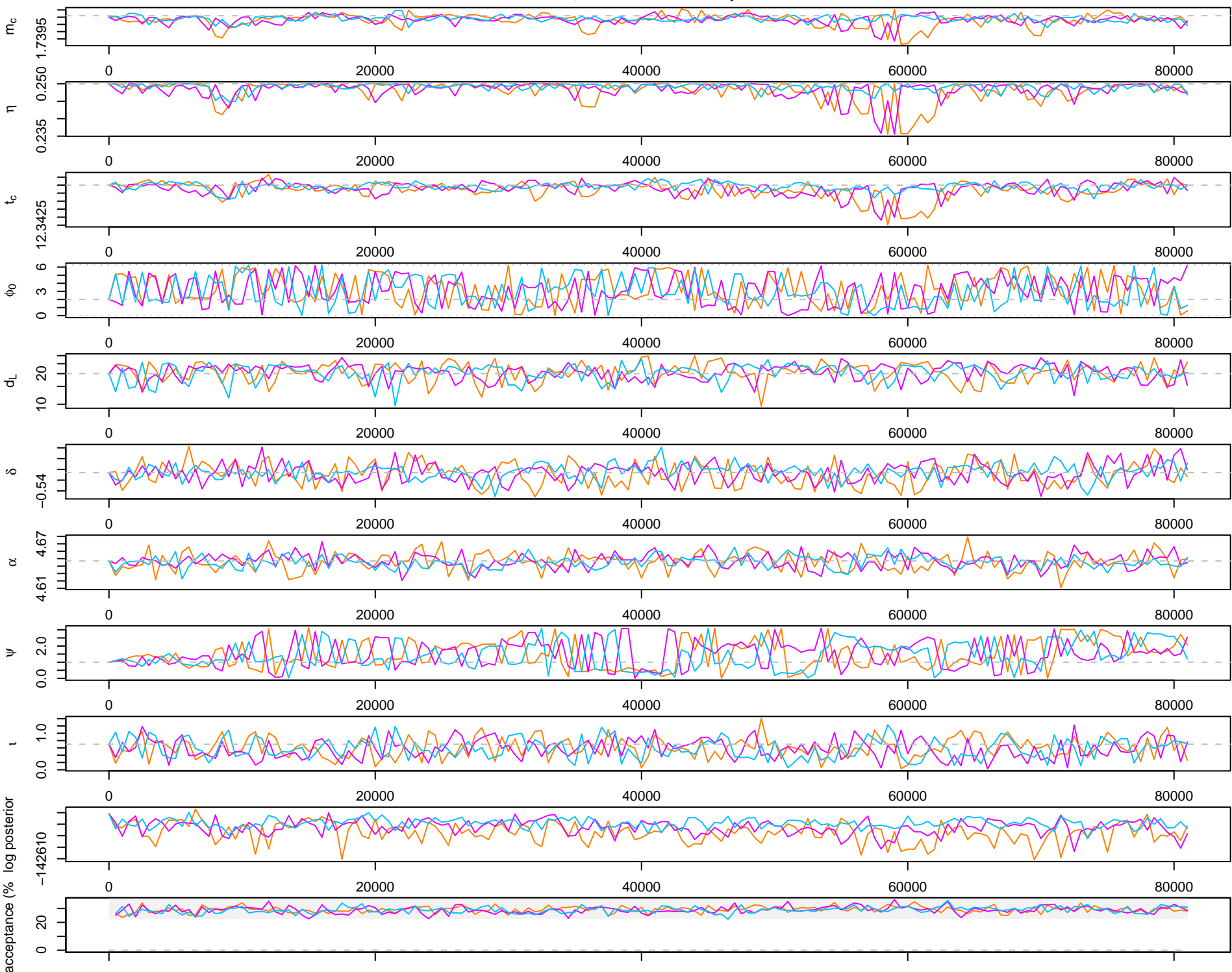
81000 iterations, 163 draws from 3 parallel chains.
