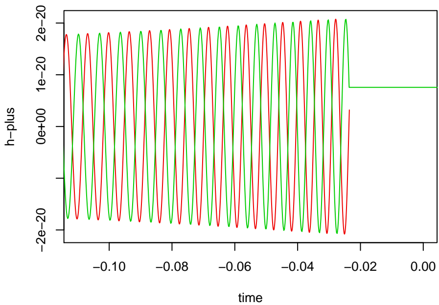
1.4 – 9.0 sun mass inspiral, \iota=0^\circ
