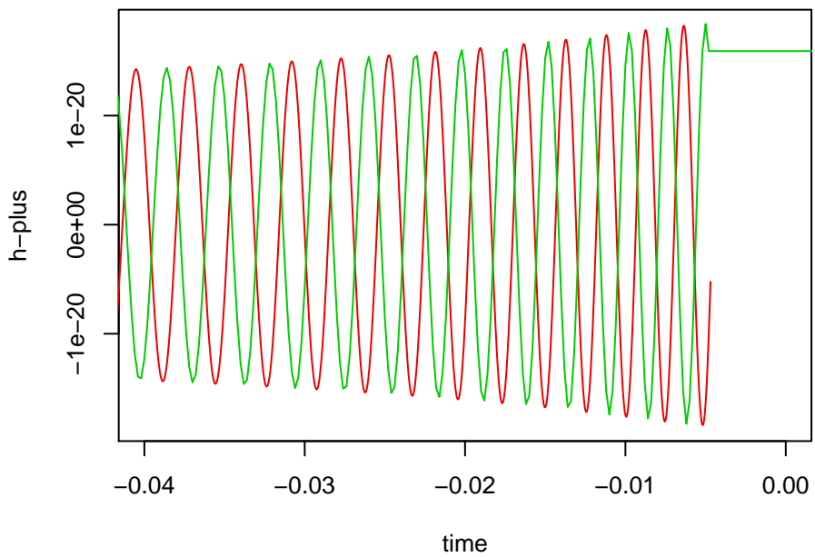
1.4 – 3.5 sun mass inspiral, \iota=0^\circ
