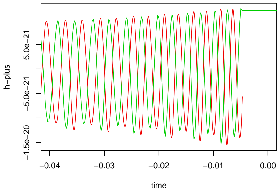
1.4 – 3.5 sun mass inspiral, \iota=45^\circ
