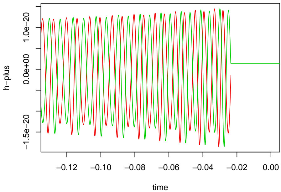
1.4 – 9.0 sun mass inspiral, \iota=45^\circ , \text{phase}=0
