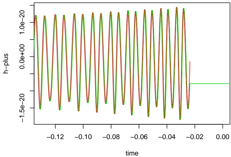
1.4 – 9.0 sun mass inspiral, \iota=45^\circ , \text{phase}=\pi/2
