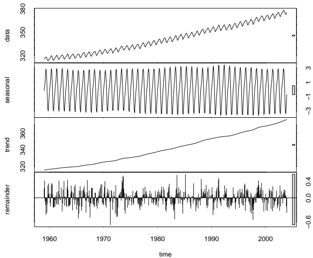
Atmospheric CO 2 (ppm) Measured at Mauna Loa
