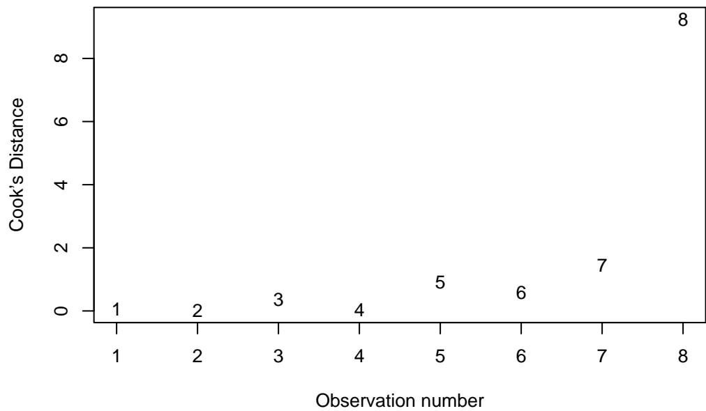
Cook's Distance Plot
