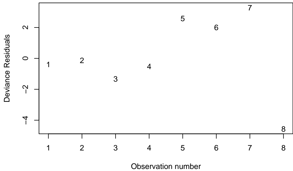
Index plot of deviance residuals
