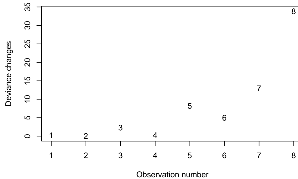
Deviance Changes Plot
