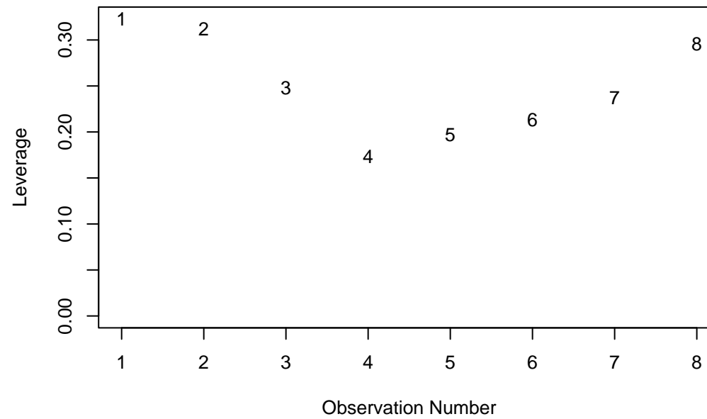
Leverage plot
