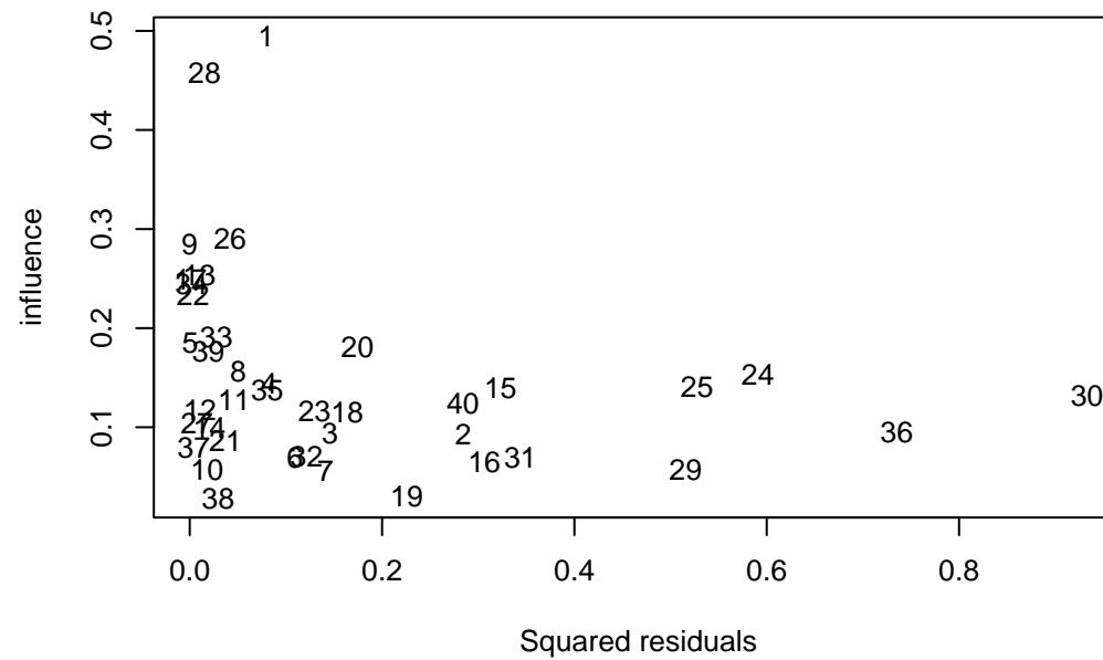
Leverage-residual plot
