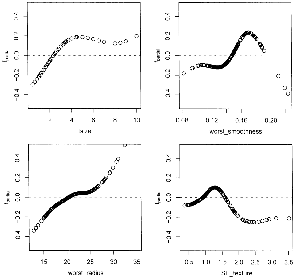
FIG. 9. wpcbc data: Partial contributions of four selected covariates in an additive logistic model (without centering of estimated functions to mean zero).
