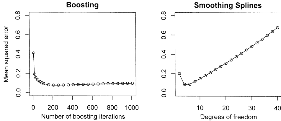
FIG. 5. Mean squared prediction error \mathbb{E}[(f(X) - \hat{f}(X))^2] for the regression model Y_i = 0.8X_i + \sin(6X_i) + \varepsilon_i ( i = 1, \dots, n = 100 ), with \varepsilon \sim \mathcal{N}(0, 2) , X_i \sim \mathcal{U}(-1/2, 1/2) , averaged over 100 simulation runs. Left: L_2 Boosting with smoothing spline base procedure (having fixed degrees of freedom df = 4 ) and using \nu = 0.1 , for varying number of boosting iterations. Right: single smoothing spline with varying degrees of freedom.
