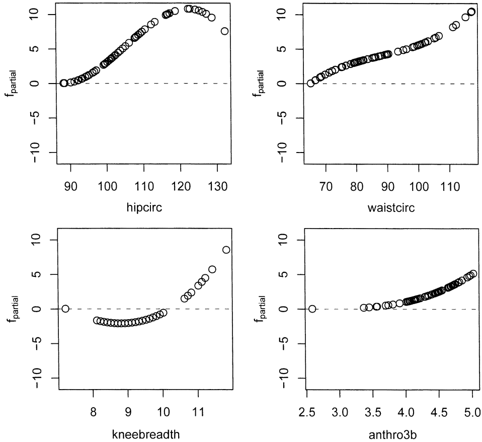
FIG. 7. bodyfat data: Partial fits for a linear model fitted to transformed covariates using B-splines (without centering of estimated functions to mean zero).
