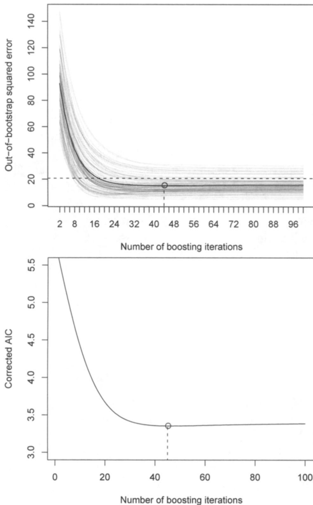
FIG. 2. bodyfat data: Out-of-bootstrap squared error for varying number of boosting iterations m_{\text{stop}} (top). The dashed horizontal line depicts the average out-of-bootstrap error of the linear model for the preselected variables hipcirc, kneebreadth and anthro3a fitted via ordinary least squares. The lower part shows the corrected AIC criterion.
