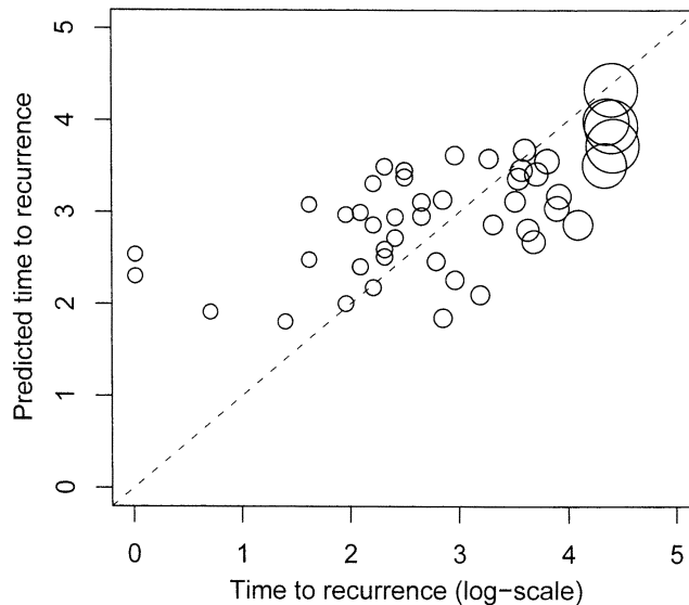
FIG. 10. wpbc data: Fitted values of an IPC-weighted linear model, taking both time to recurrence and censoring information into account. The radius of the circles is proportional to the IPC weight of the corresponding observation; censored observations with IPC weight zero are not plotted.
