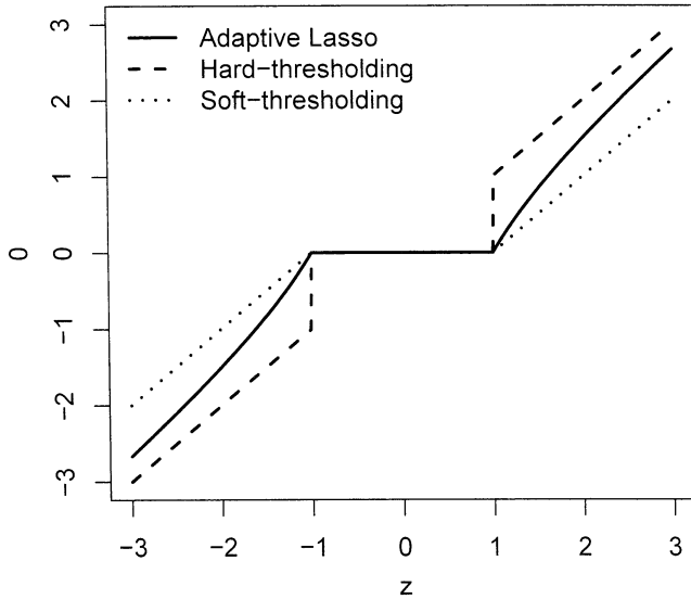
FIG. 8. Hard-threshold (dotted-dashed), soft-threshold (dotted) and adaptive Lasso (solid) estimator in a linear model with orthonormal design. For this design, the adaptive Lasso coincides with the nonnegative garrote [13]. The value on the x-abcissa, denoted by z , is a single component of \mathbf{X}^T \mathbf{Y} .
