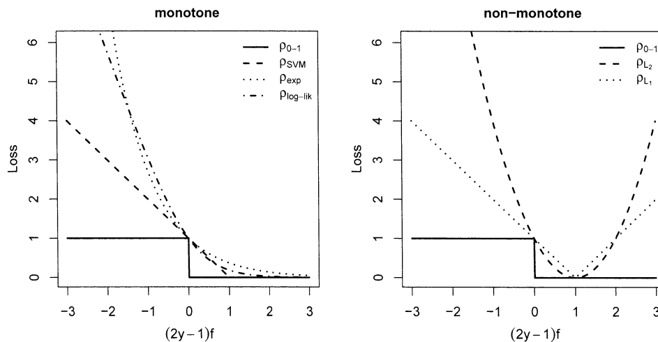
FIG. 1. Losses, as functions of the margin \tilde{y}f = (2y - 1)f , for binary classification. Left panel with monotone loss functions: 0-1 loss, exponential loss, negative log-likelihood, hinge loss (SVM); right panel with nonmonotone loss functions: squared error ( L_2 ) and absolute error ( L_1 ) as in (3.5).
