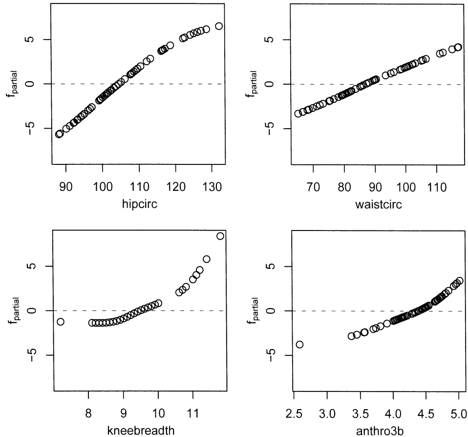
FIG. 3. bodyfat data: Partial contributions of four covariates in an additive model (without centering of estimated functions to mean zero).
