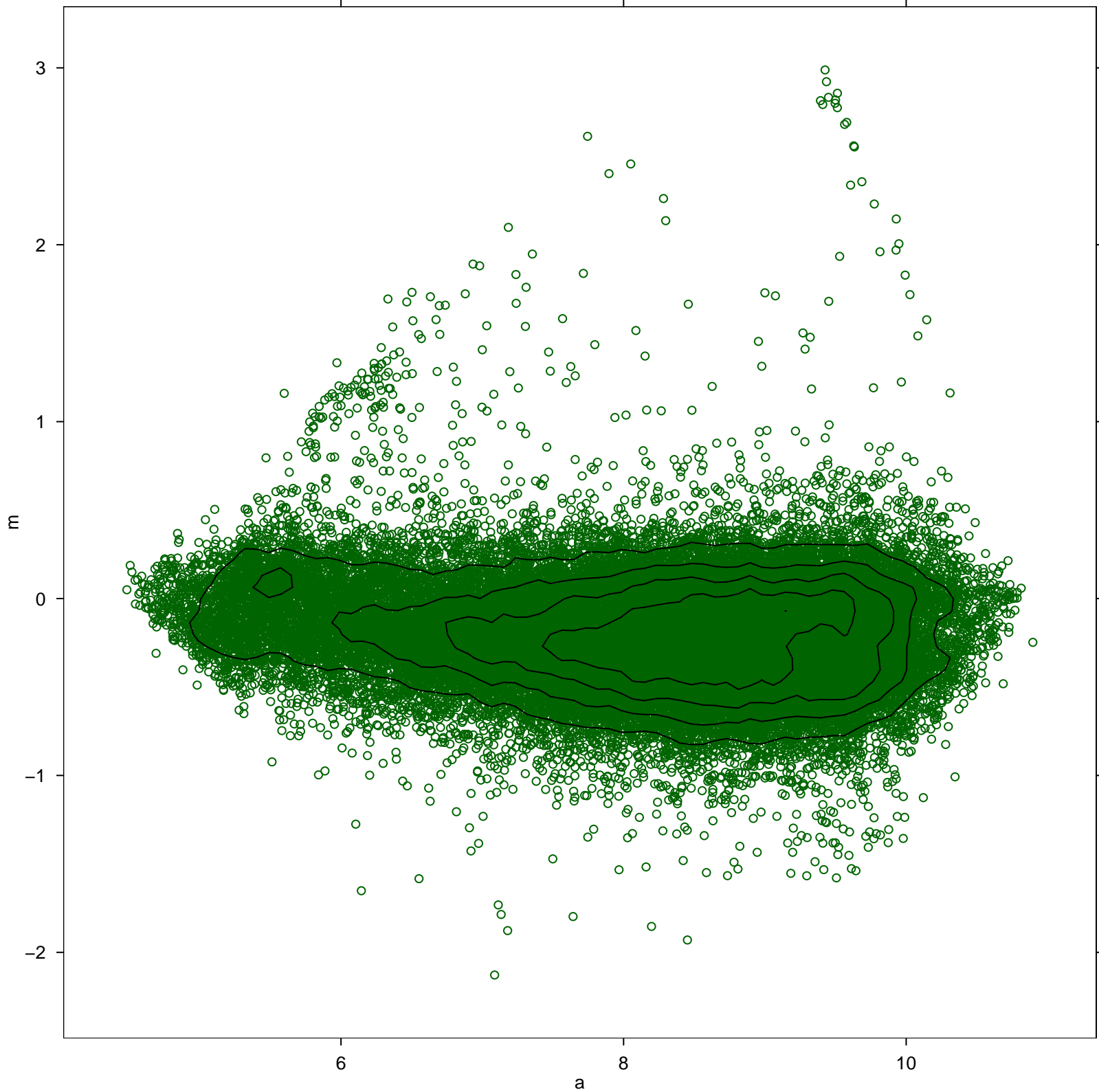
MA plot with density contours
